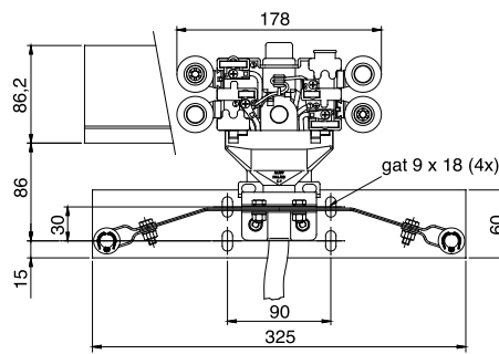
CL7-7-35 + MVSP
