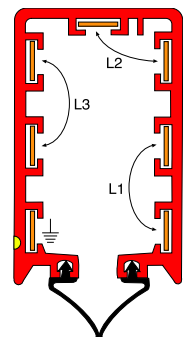
RN7-7-160/parallel
