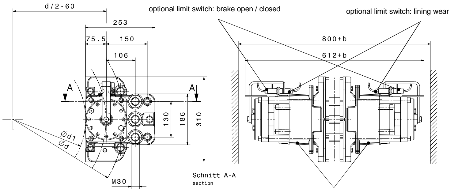
hydraulic connection M16x1.5
